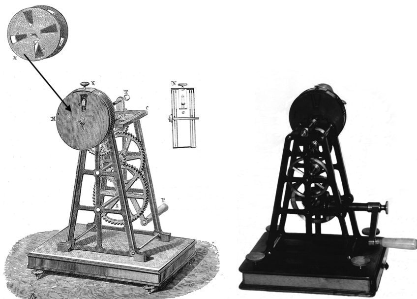
Figure 1.5 Edmond Becquerel's phosphorescope. 13) The speed of rotation of both disks bearing four windows can reach 3000 revolutions/s, which allowed analyzing
