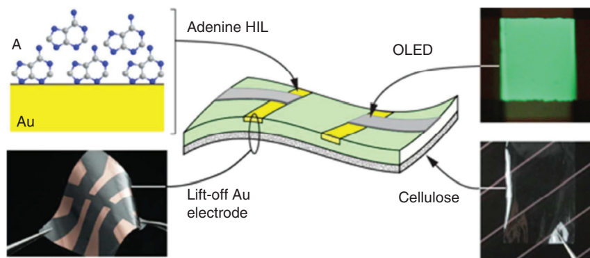
Figure 1.17 Device structure of an OLED with cellulose substrate, gold electrode, and adenine as hole injection layer. (Gomez and Steckl 2015 [61]. Reproduced with permission of American Chemical Society.)
