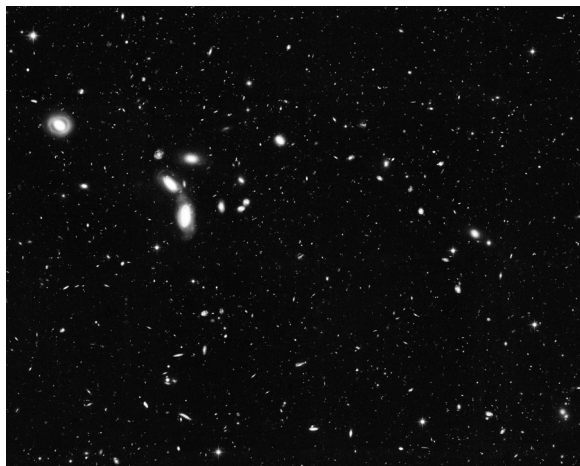
Figure 1.17 In between galaxies, there are small volumes of a few \text{dm}^3 without any massive particle (absolute or ideal vacuum). Oldest known galaxies pictured by the Hubble Space Telescope. (Courtesy of NASA.)
