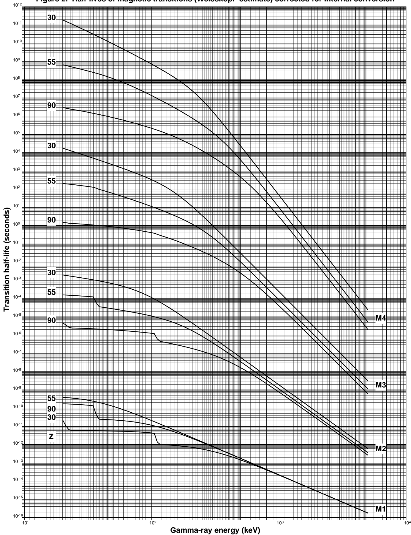
Figure 2. Half-lives of magnetic transitions (Weisskopf estimate) corrected for internal conversion
