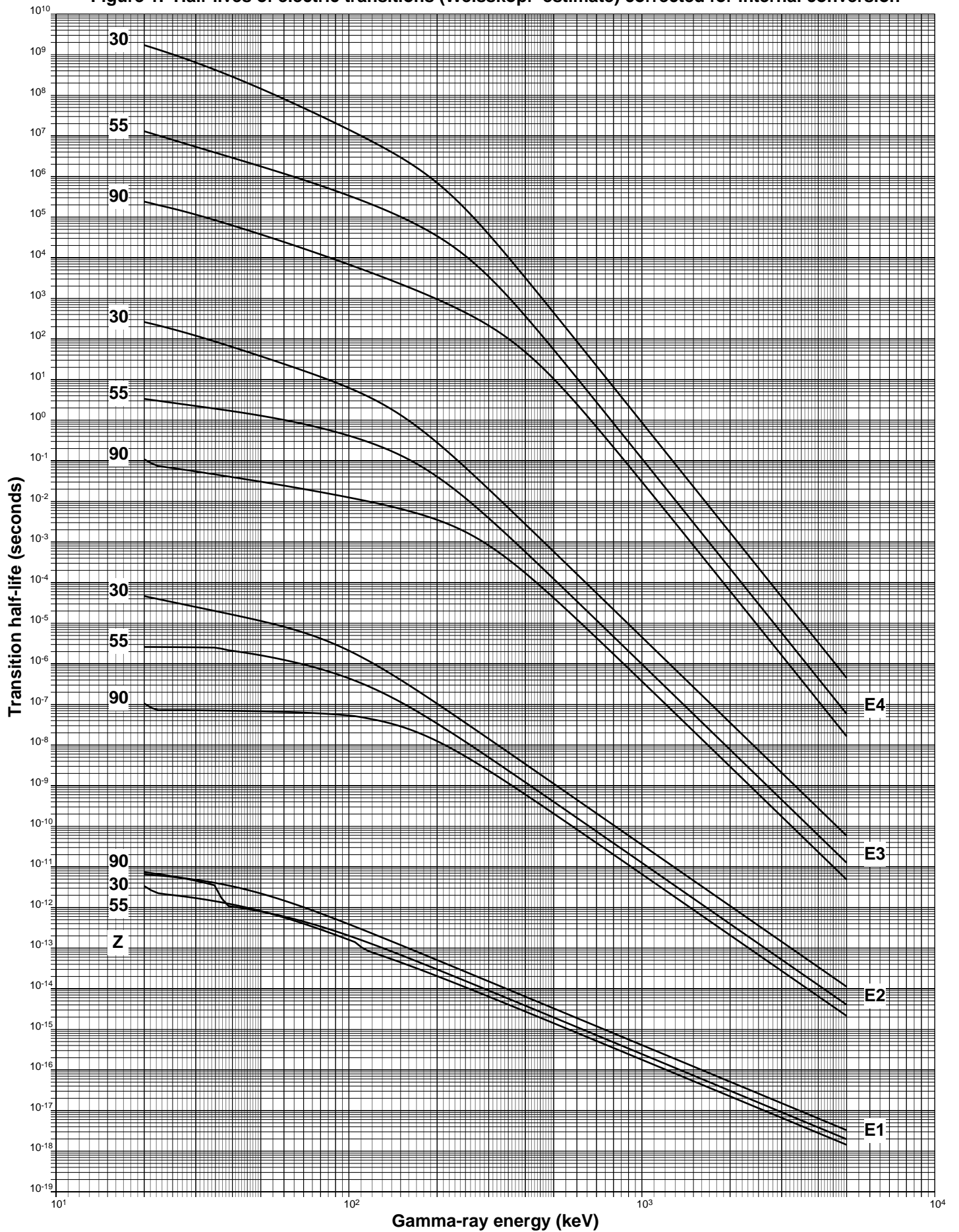
Figure 1. Half-lives of electric transitions (Weisskopf estimate) corrected for internal conversion
