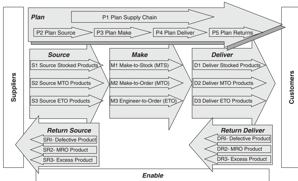
Fig. 1.2 The configuration level of the SCOR-model [12].
