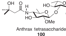
Scheme 1.19 Retrosynthesis of anthrax tetrasaccharide 100 .
