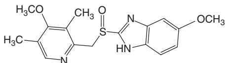
Figure 1.24 Structure of omeprazole.
