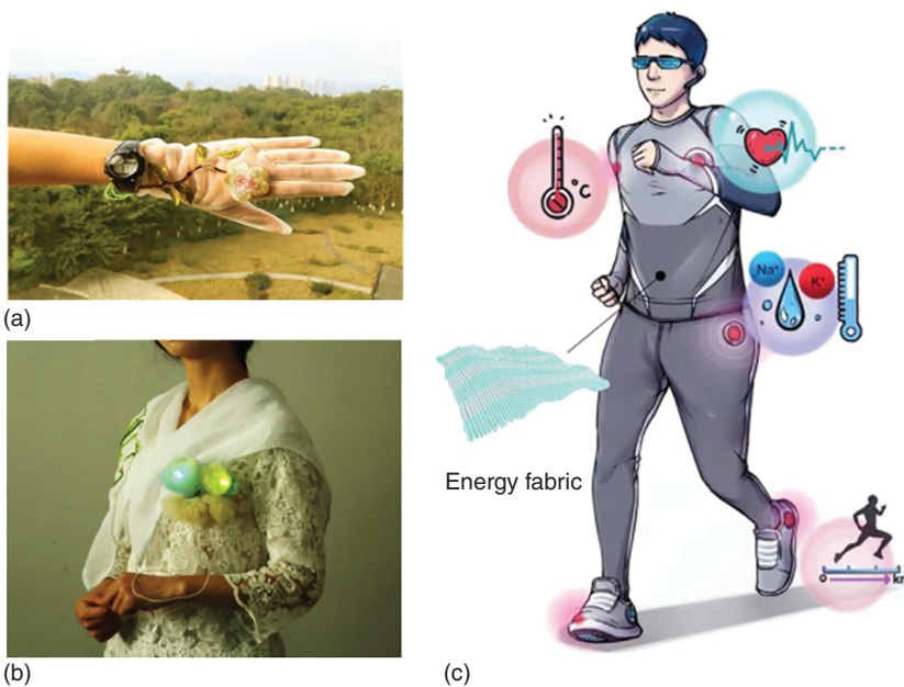
Figure 1.22 Integration of electronic devices into textiles. Demonstration of the energy fabric to serve as the power source for various portable electronics. (a) Electronic watch and (b) light-emitting diode (LED) lights. Source: Huang et al. [16]. (c) Illustration of an autonomous body area sensor network. Source: Zhang et al. [17]. © 2020, Elsevier.
