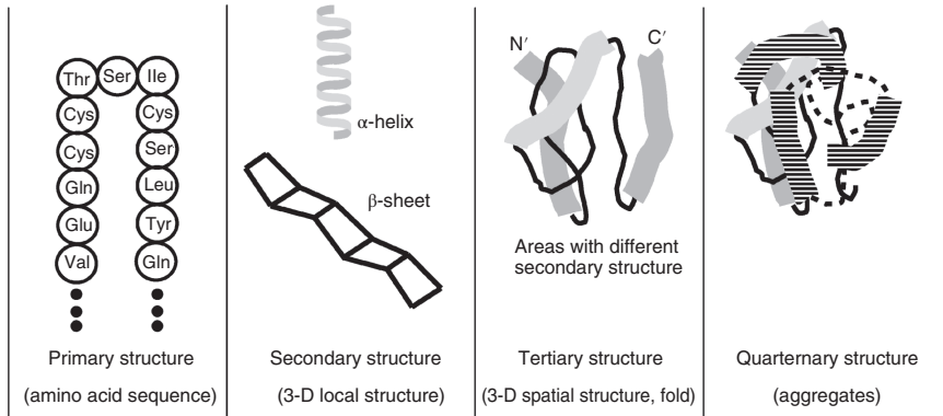
Figure 1.13 Protein structures.
