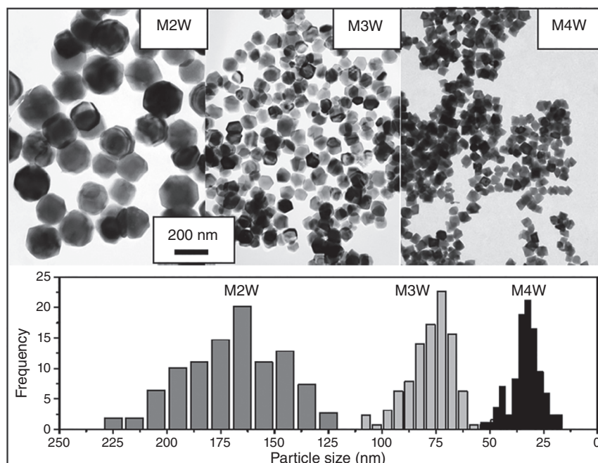
Figure 1.6 TEM images and histograms for magnetite nanoparticles synthesized at different Fe (II) concentrations. M2W, M3W, and M4W are synthesized with different ratios of [\text{Fe(II)}]:2[\text{OH}^-] , i.e. 0.997, 0.97, and 0.77, respectively, yielding average sizes of 169, 76, and 33 nm, respectively. With increasing values of the ratio, the particle shape transitions from cubic to octahedral. Source: [34] / IOP Publishing.
