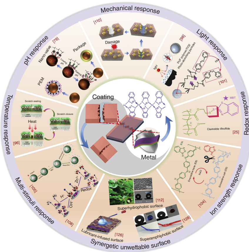
Figure 1.5 Release of corrosion inhibitors from containers in response to different stimuli. Source: Fu et al. [80]/with permission of Elsevier.
