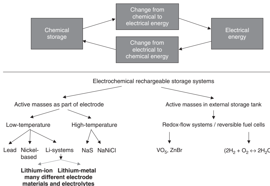
Figure 1.2 Overview of the functional principle of batteries and various materials. For details, see chapters 12–14.
