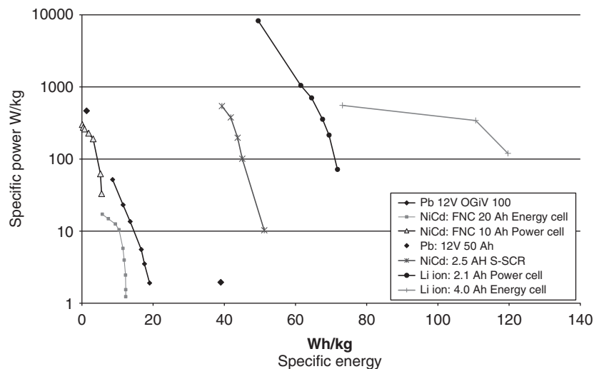
Figure 1.3 Ragone diagram of various battery technologies based on data sheet information (see Ref. [2] for further details).
