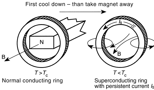
Fig. 1.1 The generation of a permanent current in a superconducting ring.
