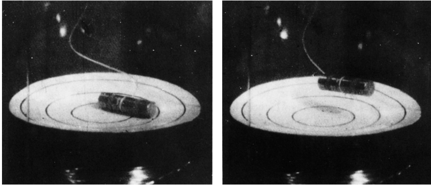
Fig. 1.7 “Levitated magnet” for demonstrating the Meissner-Ochsenfeld effect in the presence of an applied magnetic field. Left: starting position at T > T_c . Right: equilibrium position at T < T_c .
