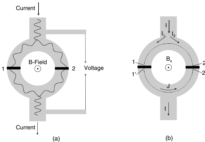
Fig. 1.24 Generation of spatial interferences of the superconducting wave function in a ring structure. (a) Schematics of the wave. (b) Notation for the derivation of the quantum interference.
