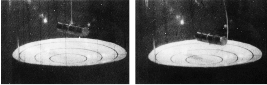
Fig. 1.3 The “levitated magnet” for demonstrating the permanent currents that are generated in superconducting lead by induction during the lowering of the magnet. Left: starting position. Right: equilibrium position.
