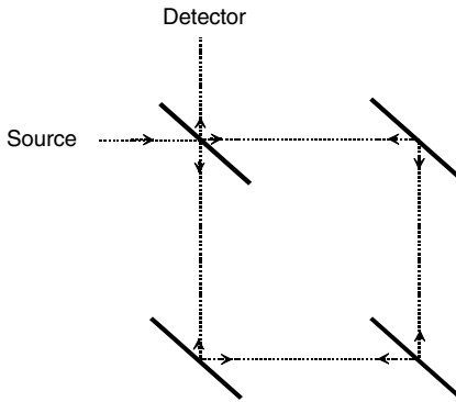
Fig. 1.18 The optical Sagnac interferometer.
