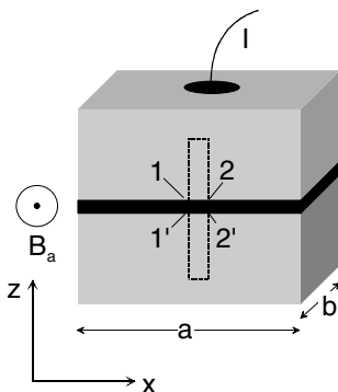
Fig. 1.26 Geometry of the spatially extended Josephson junction.
