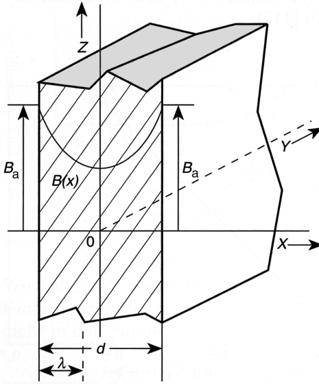
Fig. 1.15 Spatial dependence of the magnetic field in a thin superconducting layer of thickness d . For the assumed ratio d/\lambda_L = 3 , the magnetic field only decreases to about half of its outside value.
