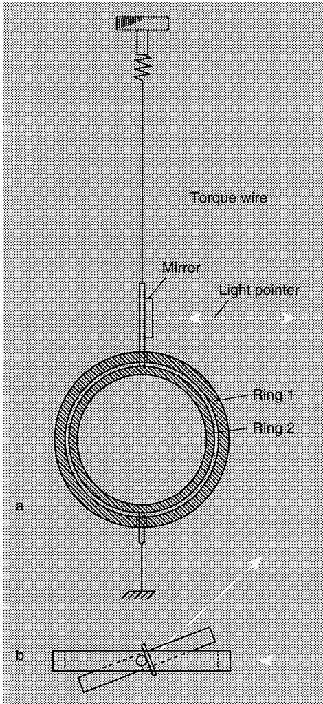
Fig. 1.2 Arrangement for the observation of a permanent current (after [2]). Ring 1 is attached to the cryostat.
