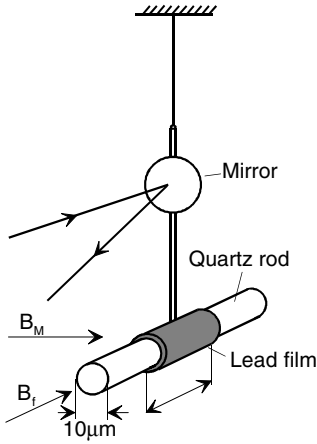
Fig. 1.11 Schematics of the experimental setup of Doll and Näbauer (from [23]). The quartz rod carries a small lead cylinder formed as a thin layer by evaporation. The rod vibrates in liquid helium.
