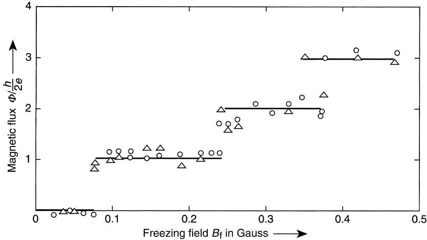
Fig. 1.13 Results of Deaver and Fairbank on the magnetic flux quantization in a Sn cylinder. The cylinder was about 0.9 mm long, and had an inner diameter of 13 \mu\text{m} and a wall thickness of 1.5 \mu\text{m} (from [24]). ( 1 \text{ G} = 10^{-4} \text{ T} ).
