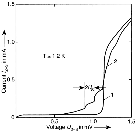
Fig. 1.23 Characteristic of the junction 2–3 from Fig. 1.22. Curve 1: no voltage at junction 1–2. Curve 2: 0.055 mV applied to junction 1–2.
