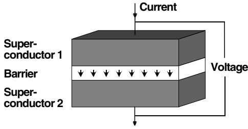
Fig. 1.19 Sandwich geometry of two superconductors separated from each other by a thin barrier.
