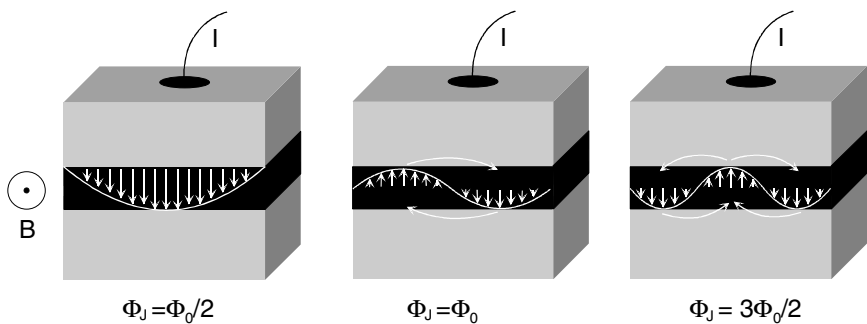
Fig. 1.28 Variation of the Josephson supercurrent density for three different values of the magnetic flux penetrating through the Josephson junction.
