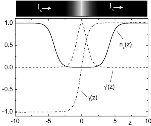
Fig. 1.20 Derivation of the Josephson equations. We consider a thin superconducting wire with a weakened location at z = 0 , at which the Cooper pair density n_s is strongly reduced. Due to current conservation, we have n_s(z)\gamma'(z) = \text{const.} , leading to a peak in \gamma'(z) and to a step in \gamma . For illustration we have used the following “test function”: n_s(z) = 1/\gamma'(z) = 1/[1.001 - \tanh^2(x)] , \text{const.} = 0.001 . For \gamma(z) one finds \gamma(z) = \tanh(z) + 0.001z . At the weakened location \gamma(z) changes very rapidly from -1 to +1 .
