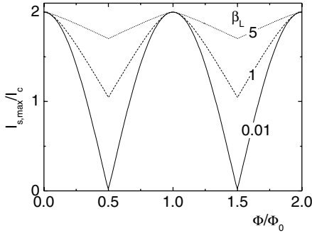
Fig. 1.25 Modulation of the maximum supercurrent of a superconducting quantum interferometer as a function of the magnetic flux through the ring. The curves are shown for three different values of the inductance parameter \beta_L .
