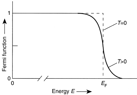
Fig. 1.6 Fermi function. E_F is a few eV, whereas thermal smearing is only a few 10^{-3} eV. To indicate this, the abscissa is interrupted.
