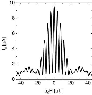
Fig. 1.29 Magnetic field dependence of the maximum supercurrent of a SQUID structure made of \text{YBa}_2\text{Cu}_3\text{O}_7 . The two Josephson junctions are 9\ \mu\text{m} wide, such that the I_c modulation of the individual junctions appears as the envelope of the SQUID oscillations [54] (© 2000 AIP).
