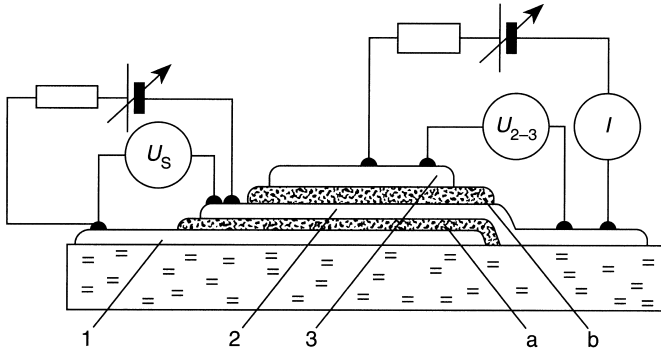
Fig. 1.22 Arrangement for the experimental demonstration of the alternating Josephson current according to Giaever: layers 1, 2, and 3 are Sn layers; layers a and b are oxide layers. The thicknesses of layers a and b are chosen such that layers 1 and 2 form a Josephson junction, and such that no Josephson currents are possible between layers 2 and 3 (from [42]).
