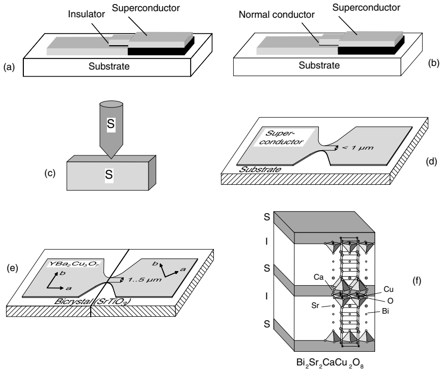
Fig. 1.21 Schematics of the different possibilities for producing a weak coupling between two superconductors: (a) SIS junction with an oxide layer as a barrier; (b) SNS junction with a normal conducting barrier; (c) point contact; (d) microbridge; (e) \text{YBa}_2\text{Cu}_3\text{O}_7 grain boundary junction; (f) intrinsic Josephson junction in \text{Bi}_2\text{Sr}_2\text{CaCu}_2\text{O}_8 .
