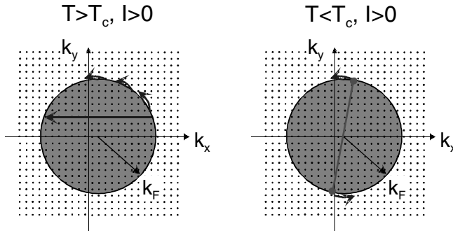
Fig. 1.17 Generation of the supercurrent: current transport and decay of the permanent current illustrated with the Fermi sphere.
