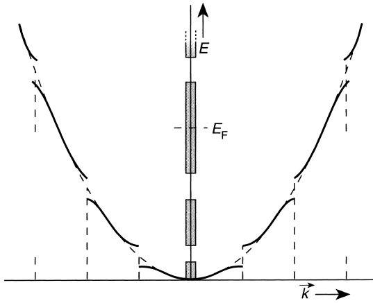
Fig. 1.5 Energy-momentum relation for an electron in a periodic potential. The relation (Eq. 1.2) valid for free electrons is shown as the dashed parabolic line.
