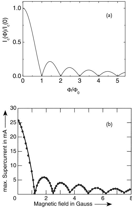
Fig. 1.27 Dependence of the maximum Josephson current on the magnetic field parallel to the barrier layer. (a) Theoretical curve according to Eq. (1.73). (b) Measured data for a Sn-SnO-Sn tunnel junction (from [53]). ( 1 \text{ G} = 10^{-4} \text{ T} ).
