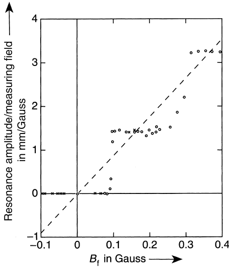
Fig. 1.12 Results of Doll and Näbauer on the magnetic flux quantization in a Pb cylinder (from [23]). ( 1 \text{ G} = 10^{-4} \text{ T} ).
