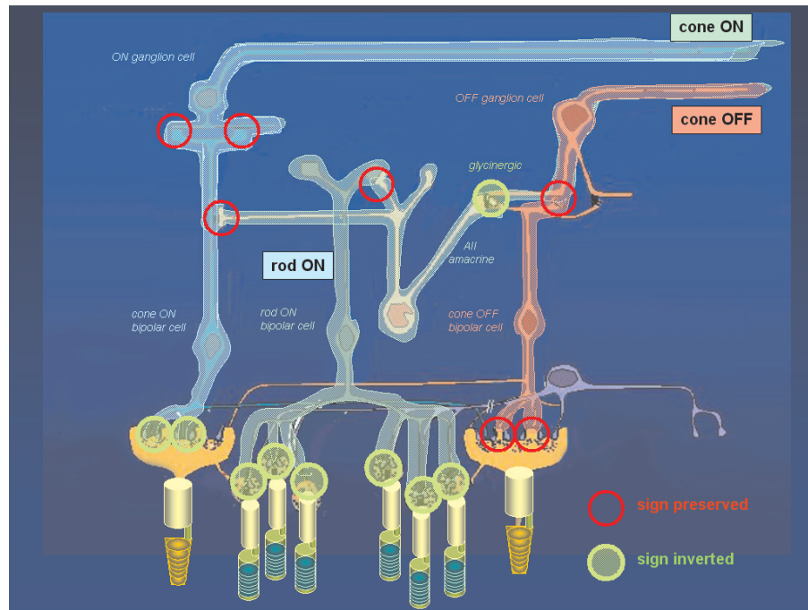
Fig. 1.10 Rod and cone pathways and ON/OFF channels. To make the system more sensitive to differences, rather than to absolute brightness, the image on the retina is analyzed by an ON/OFF system, i.e., cells that respond preferably by changes in brightness in either direction. The division into these two major channels occurs already at the first synapse, the photoreceptor endfoot . Because the photoreceptors can only hyperpolarize in response to illumination, the subsequent cells must be either depolarized ( excited ) or hyperpolarized ( inhibited ). This means that the signal must either be inverted ( ON channel ) or conserved
