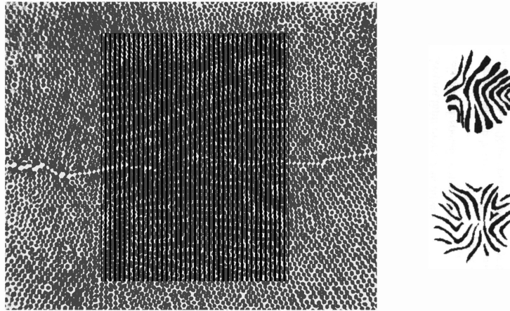
Fig. 1.6 Aliasing (undersampling) and Moiré patterns. If a grating is imaged on the photoreceptor array, and the sampling interval of the receptors is larger than half the spatial wavelength of the grating, patterns appear. The photoreceptor lattice (left) is from a histological
