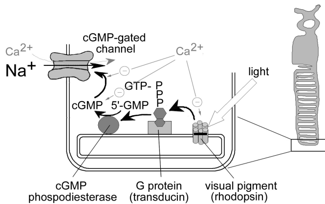
Fig. 1.8 Principle of the phototransduction cascade and the role of calcium in light/dark adaptation in a rod photoreceptor. The pigment molecule embedded in the photoreceptor outer segment disc membrane, consisting of a protein (opsin) and retinal (an aldehyde), absorbs a photon and converts into an activated state which can stimulate a G protein (transducin in rods). Transducin, in turn, activates an enzyme, cGMP phosphodiesterase, which catalyzes the breakdown of cGMP to 5'-GMP. cGMP has a key role in phototransduction: to open the cGMP-gated cation channels , 3 cGMP molecules have to bind to the channel protein. Therefore, if cGMP is removed
