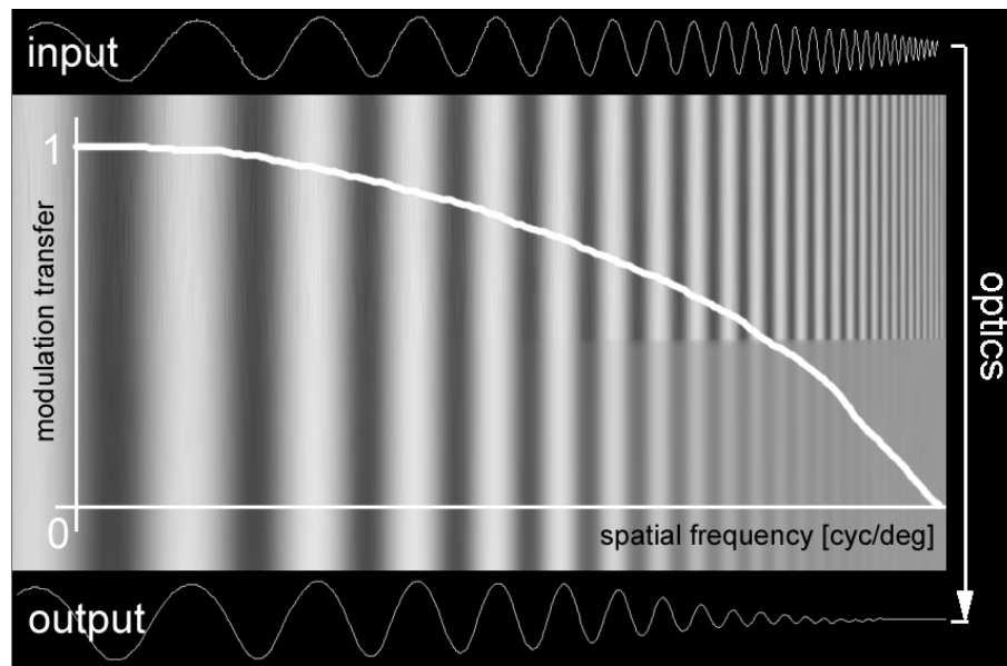
Fig. 1.3 The spatial information in an image can be reconstructed as a linear superposition of sine wave components (spatial frequencies) with different amplitudes and phases (Fourier components). Low spatial frequencies (SF) are generally available with high contrast in the natural visual environment, whereas the contrast declines for higher spatial frequencies, generally proportional to 1/\text{SF} ( input ). Due to optical imperfections and diffraction, the image on the retina does not retain the input contrast at high spatial frequencies. The decline of modulation transfer , the ratio of output to input
