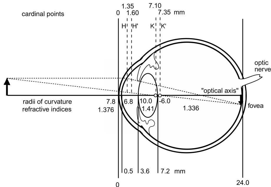
Fig. 1.1 Dimensions and schematic optics of the left human eye, seen from above. The anterior corneal surface is traditionally set to coordinate zero. All positions are given in Millimeters, relative to the anterior corneal surface (drawing not to scale). The refracting surfaces are approximated by spheres so that radii of curvatures can be defined. The cardinal points of the optical system, shown on the top, are valid only for rays close to the optical axis ( Gaussian approximation ). The focal length of the eye in the vitreous (the posterior focal length) is 24.0 mm — H = 22.65 mm. The nodal points K and K' permit us to calculate the retinal image magnification. In the first approximation, the posterior nodal distance ( PND , distance K to the focal point at the retina) determines the linear distance on the retina for a given visual angle. In the
