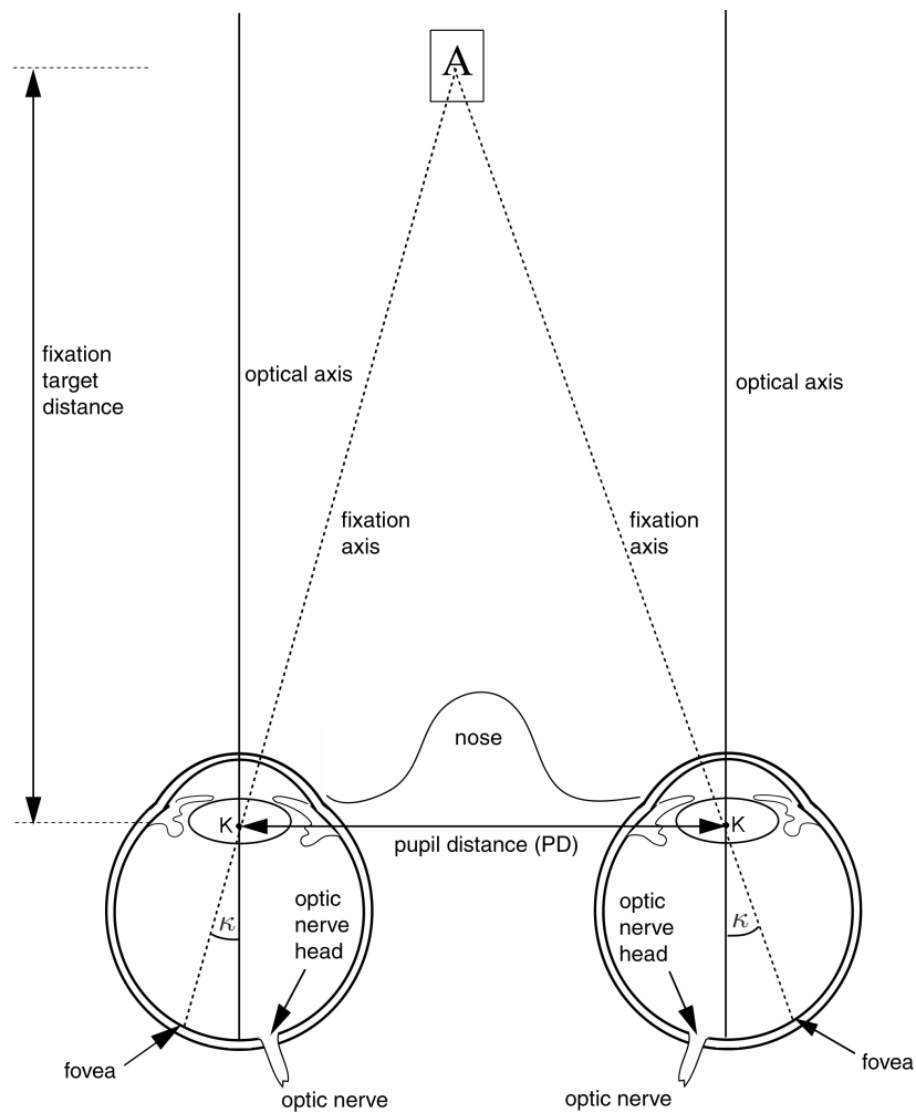
Fig. 1.2 Binocular geometry of human eyes, seen from above. Since the fovea is temporally displaced with regard to the optical axis by the angle \kappa , the optical axes of the eyes do not reflect the direction of fixation. \kappa is highly variable among eyes, ranging from zero to 11^\circ , with an average of about 3.5^\circ . In the illustrated case, the fixation target is at a distance for which the optical axes happen to be parallel and straight. The distance of the fixation target, for which this is true, can be easily calculated: for an angle \kappa of 4^\circ , a pupil distance of 64 mm, this condition
