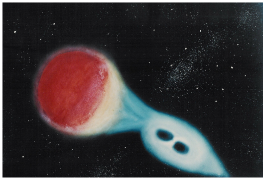
Figure 10: An artist's conception of Her X-1 with accretions occurring at the poles of the magnetic field of the neutron star. Illustration of R. Plourde.
