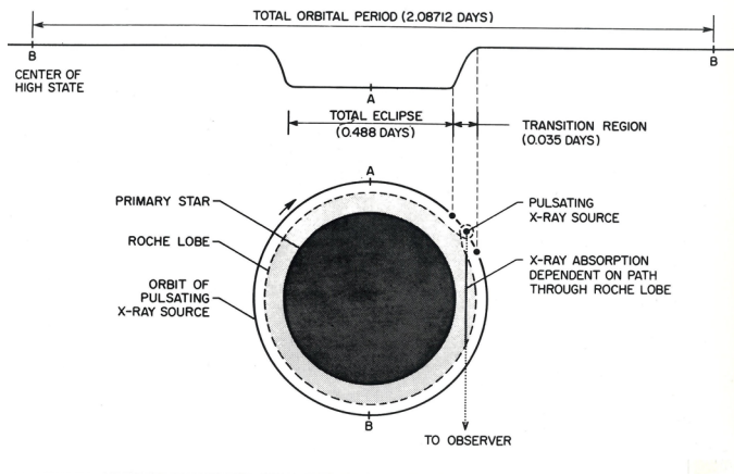
Figure 7: A model of the Cen X-3 binary system. Illustration of R. Giacconi.
