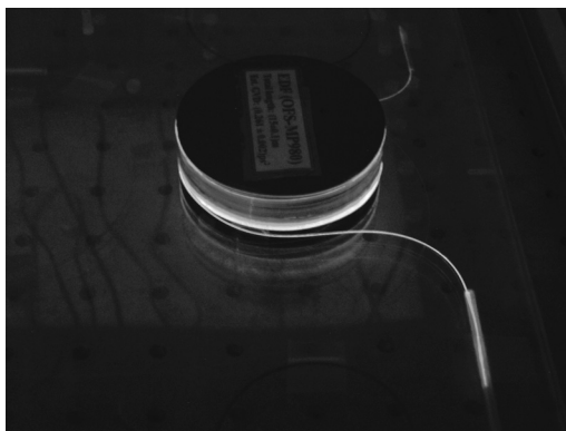
Figure 1.13 Erbium doped fiber glowing in the dark, upon excitation by the pump radiation at 980 nm. Please find a color version of this figure on the color plates.
