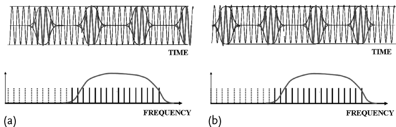
Figure 1.33 The mode-locked pulse train, in the time domain (top) is shown as a wave at a single carrier frequency, modulated by and envelope. The corresponding comb of optical frequencies is represented on the bottom. (a) A general case where the envelope spacing is not an in-
