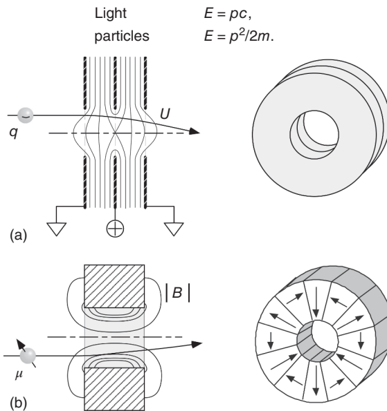
Figure 1.22 Lenses for particle optics. (a) The so-called single lens for electron optics with equipotential surfaces |qU| [4]. The potential is created by symmetric positioning of three conducting electrodes, the two outer ones lying on the same potential. (b) Magnetic lens for atom optics with equipotential surfaces |\mu \cdot B| [5, 6]. An axial magnetic hexapole is formed out of circle segments, which are manufactured from a homogeneously magnetized permanent magnet (e.g., NdFeB or SmCo). The strength of the magnetic field rises as a square function of the radial distance.
