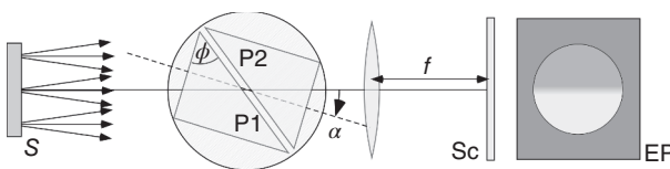
Figure 1.23 Abbe’s refractometer, illuminated with a diffusive source S . The liquid is filled in the thin gap between parallel prisms P1 and P2 . The double prism is rotated by an angle \alpha until a half-bright/half-dark image EP appears on the screen Sc . The lens has focal length f .
