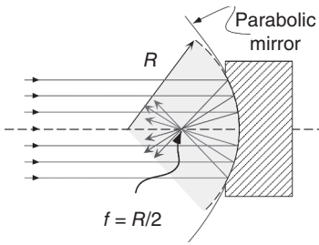
Figure 1.15 Path of rays for a concave mirror. For near-axis incident light, spherical mirrors are used. The effect on a parallel beam of rays within one cut plane is visualized in Figure 1.15.
