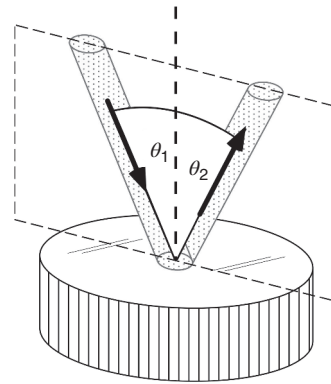
Figure 1.2 Reflection at a planar mirror.
