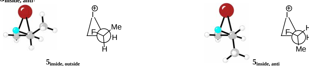
Figure 4. Most stable rotamers with fluoride and methyl substituents, 5 inside, outside and 5 inside, anti .
