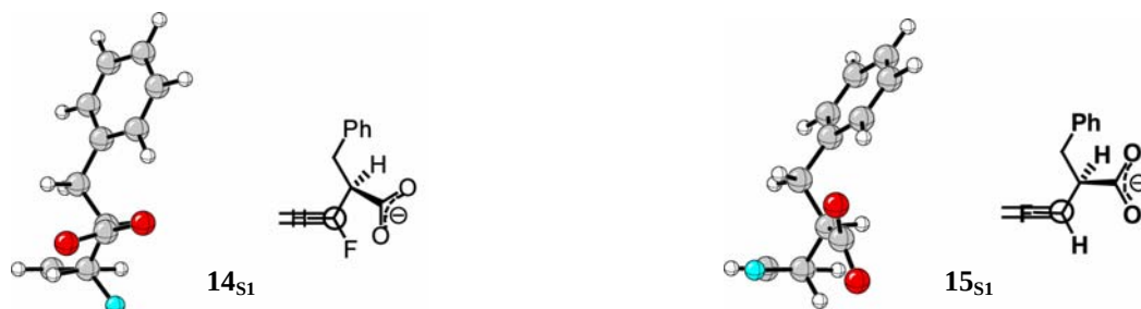
Figure 1. Most stable rotamers of 14 and 15 .
