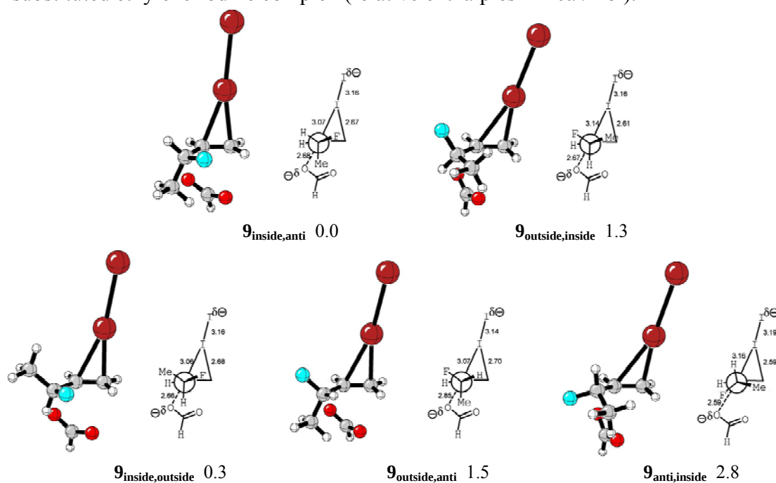
Figure 11. Intermolecular transition structure isomers for addition of formate to substituted ethylene-iodine complex (relative enthalpies in kcal/mol).
