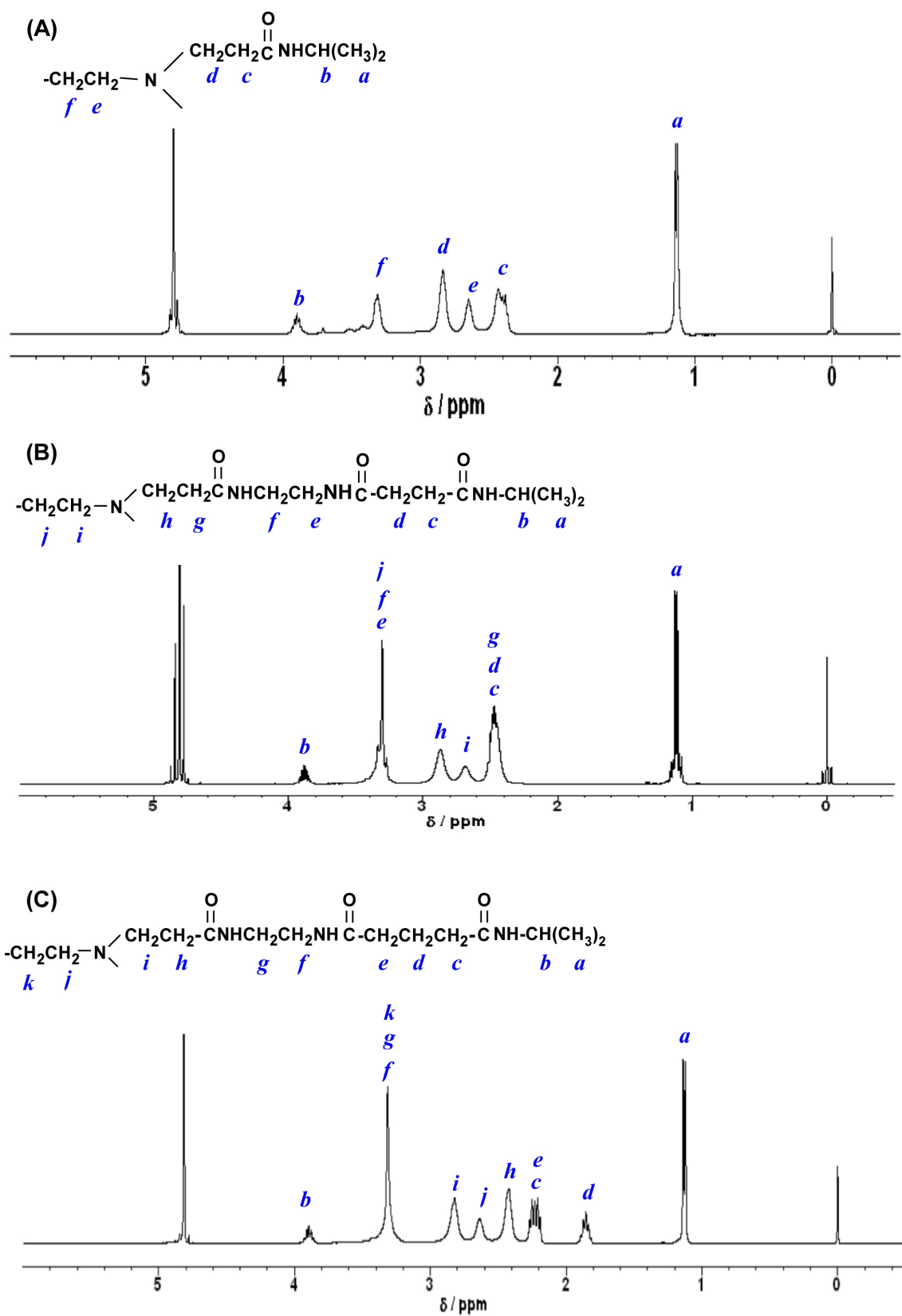
Figure S1. ^1\text{H} NMR spectra of NIPAM-0-G4.5 (A), NIPAM-3-G5 (B), and NIPAM-4-G5 (C) dendrimer in \text{D}_2\text{O}
