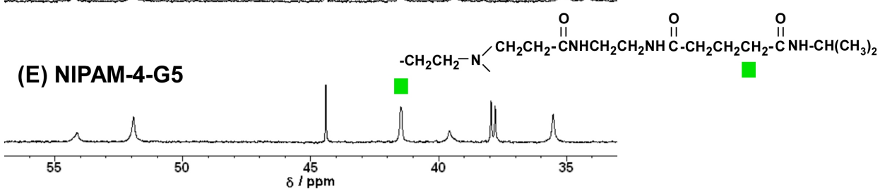
Figure S2. ^{13}\text{C} NMR spectra of PAMAM G4.5 (A), NIPAM-0G4.5 (B), PAMAM-G5 (C), NIPAM-3-G5 (D), and NIPAM-4-G5 (E) in \text{D}_2\text{O} .
