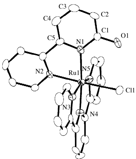
Figure S1. Molecular structure of [Ru(trpy)(bpy-OH)Cl] + with atom labeling. Hydrogen atoms are omitted for simplicity.
