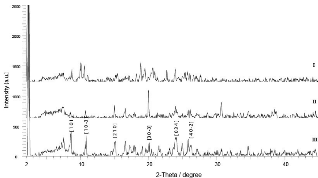
Supp. Fig.1 X-ray powder diffraction of I (triclinic, P \bar{1} ), II (monoclinic, C2/c) and III (monoclinic, P2 1 /n)
