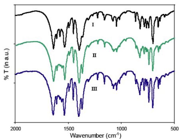
Supp. Fig.2 Solid-state FT-IR spectra (KBr, cm -1 ) of crystals of polymorphs I-III showing the C=O and N-O stretching bands
