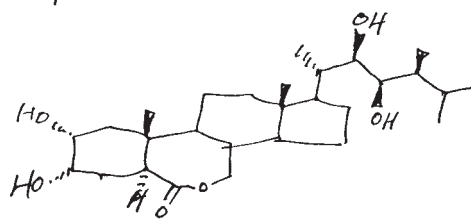
Brassinolide
