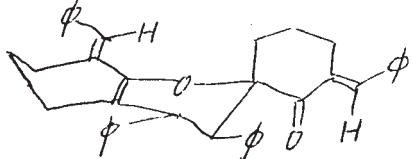
2,6-dibenzylidene-cyclohexanone dimer
