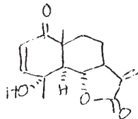
Arglamine
