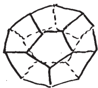
Dodecahedrane
