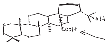
PHEBIC ACID C
