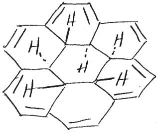
Heptahydrocoronene
