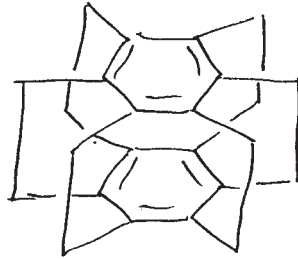
superphane
