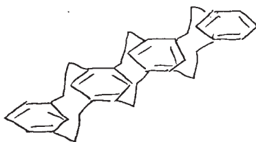
Quadruple-layered metacyclophane
