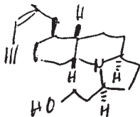
Gephyrotoxin
