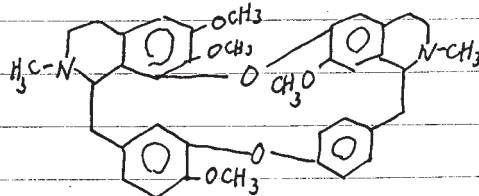
O-methylthalicberine
