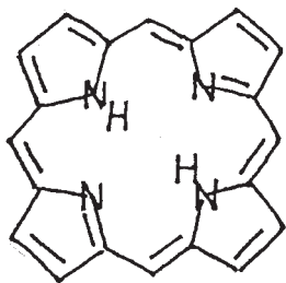
Porphin
