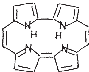
Porphycene
